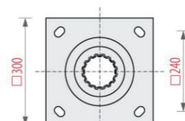
Khung móng / Anchor bolts 4/M16 x 500
